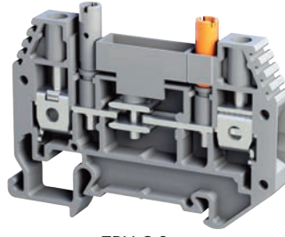
TDY-C 6
