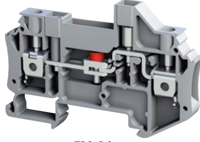
TDS-C 6
