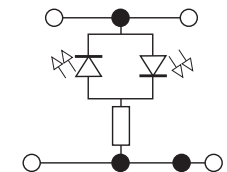
8002099368 TBL 4 2PL (24-48VAC/DC) Gri 8002099378 TBL 4 2PL (110-220VAC/DC) Gri
