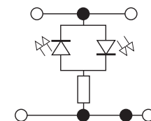
8002099368 TBL 4 2PL (24-48VAC/DC) 8002099378 TBL 4 2PL (110-220VAC/DC)
